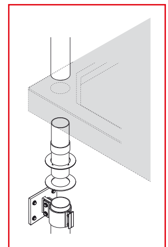
Platformsteun
